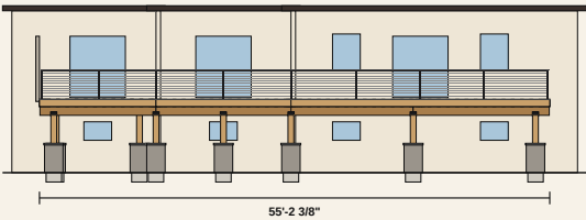
FRONT ELEVATION — from the yard
