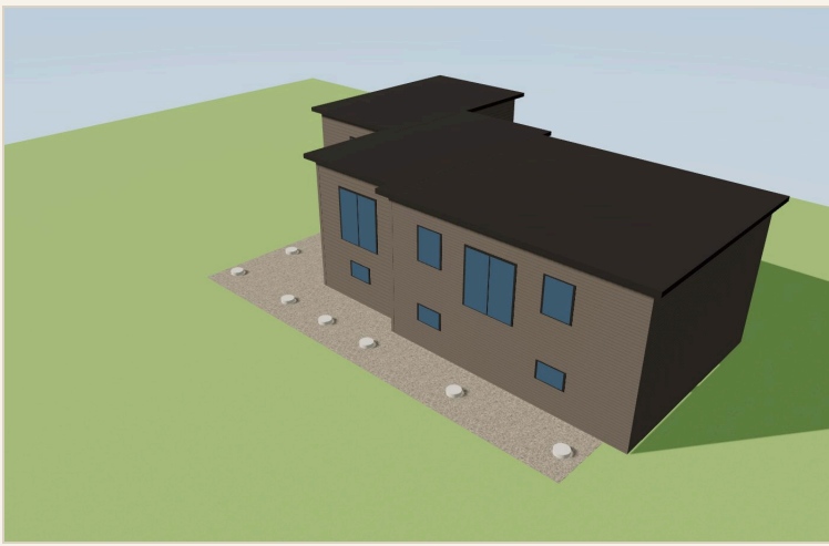
Step 1 • Footings — 8 caissons 20" x 3.5' below frost
