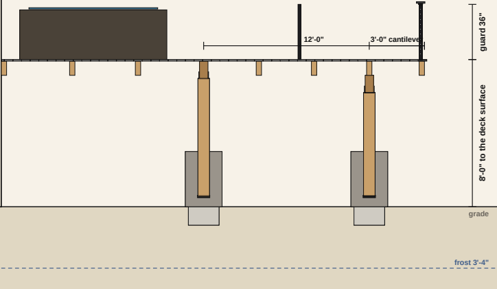
SECTION through zone C at 6'-3 5/8" — looking toward the left end
